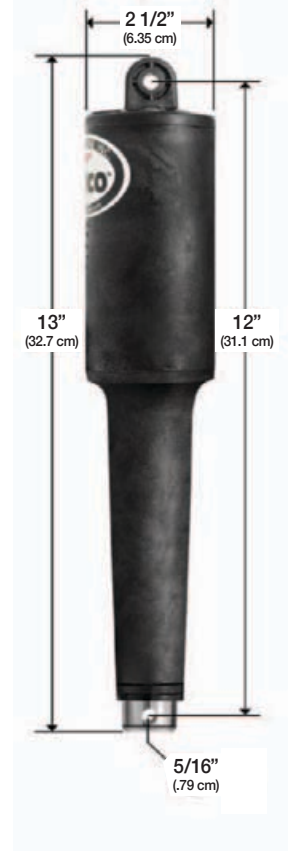
102 HD/XD Actuator 4 1/4" Stroke (10.795 cm)
