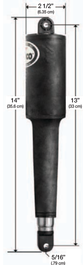
102 Actuator 4 1/4" Stroke (10.795 cm)
