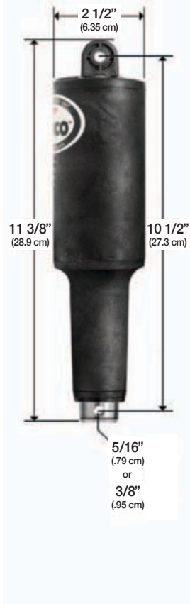
101 XD Actuator 2 1/4" Stroke (5.715 cm)
