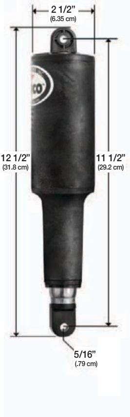
101 Standard Actuator 2 1/4" Stroke (5.715 cm)
