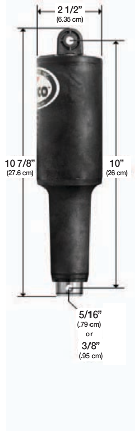
101 XDS (Short) Actuator 2 1/4" Stroke (5.715 cm)
