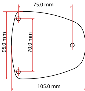
Mounting Plate Measurements
