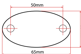
Mounting Plate Measurements
