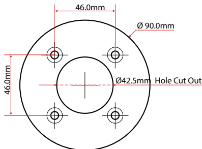
Mounting Plate Measurements
