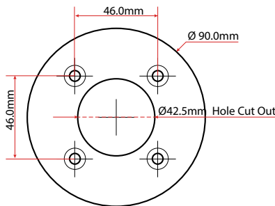
Mounting Plate Measurements
